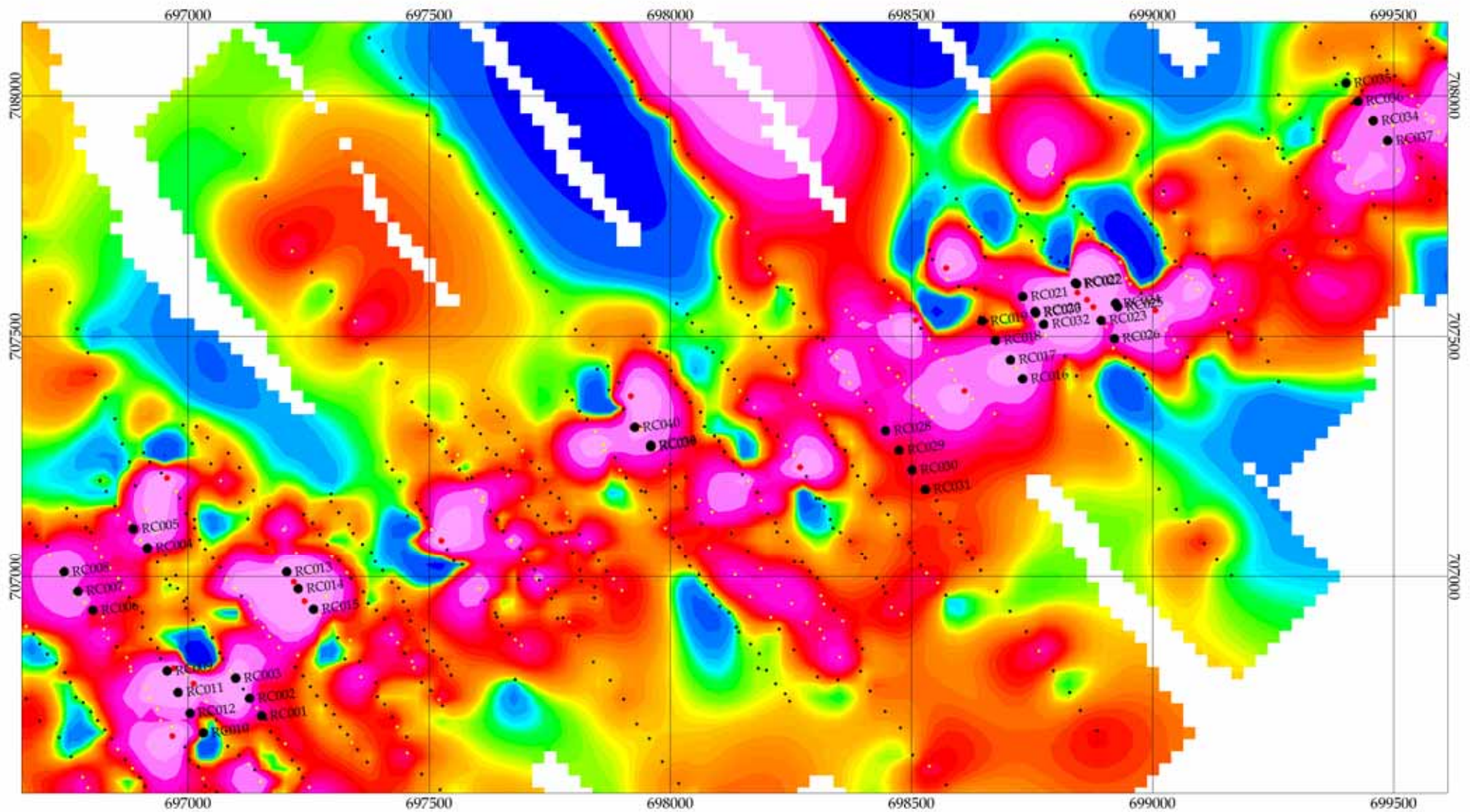
Banso Project RC Drill Hole Locations Gold Soil Geochemical Image
