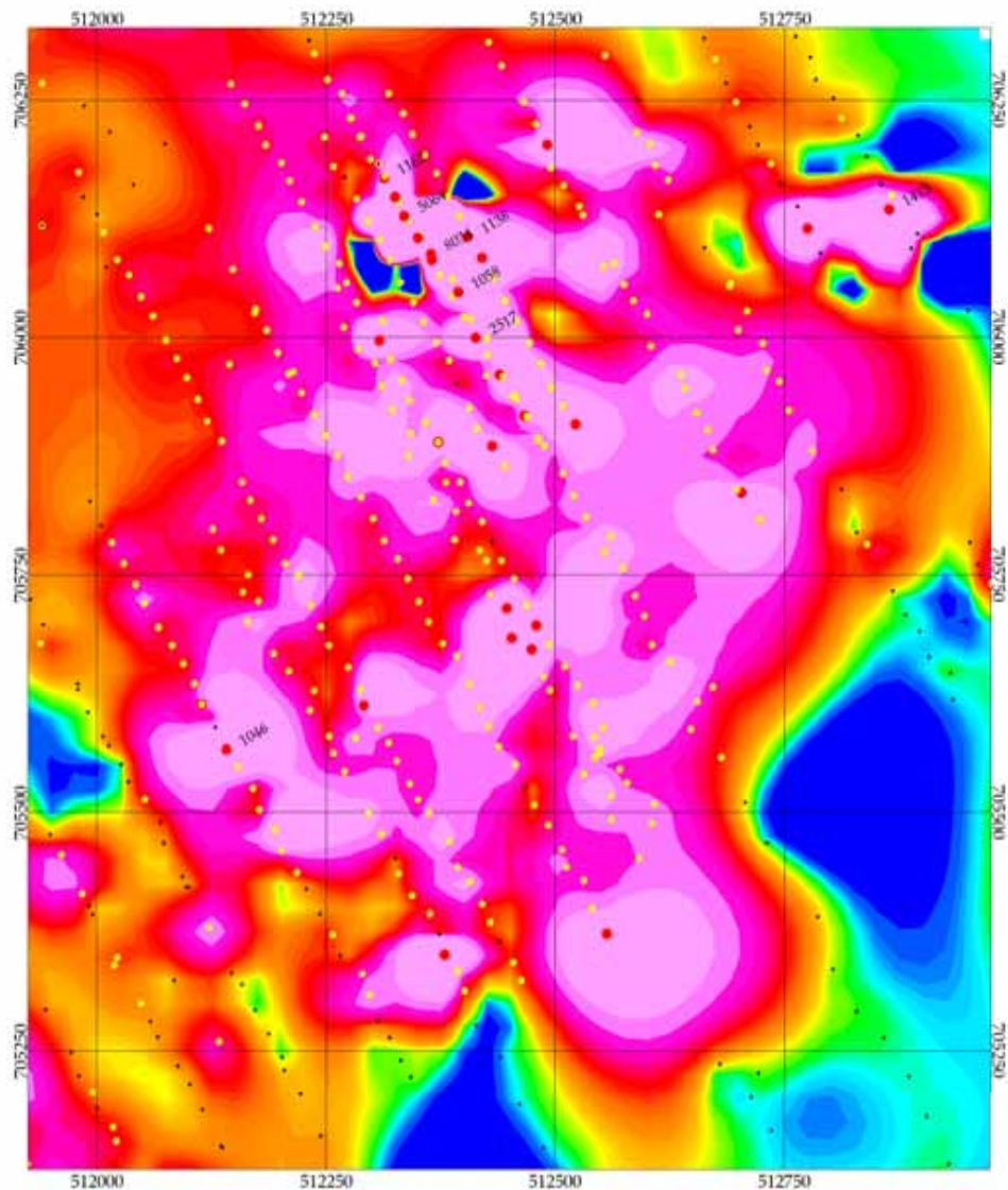
Boizan Prospect Gold Soil Geochemistry Boizan Gold Anomaly
