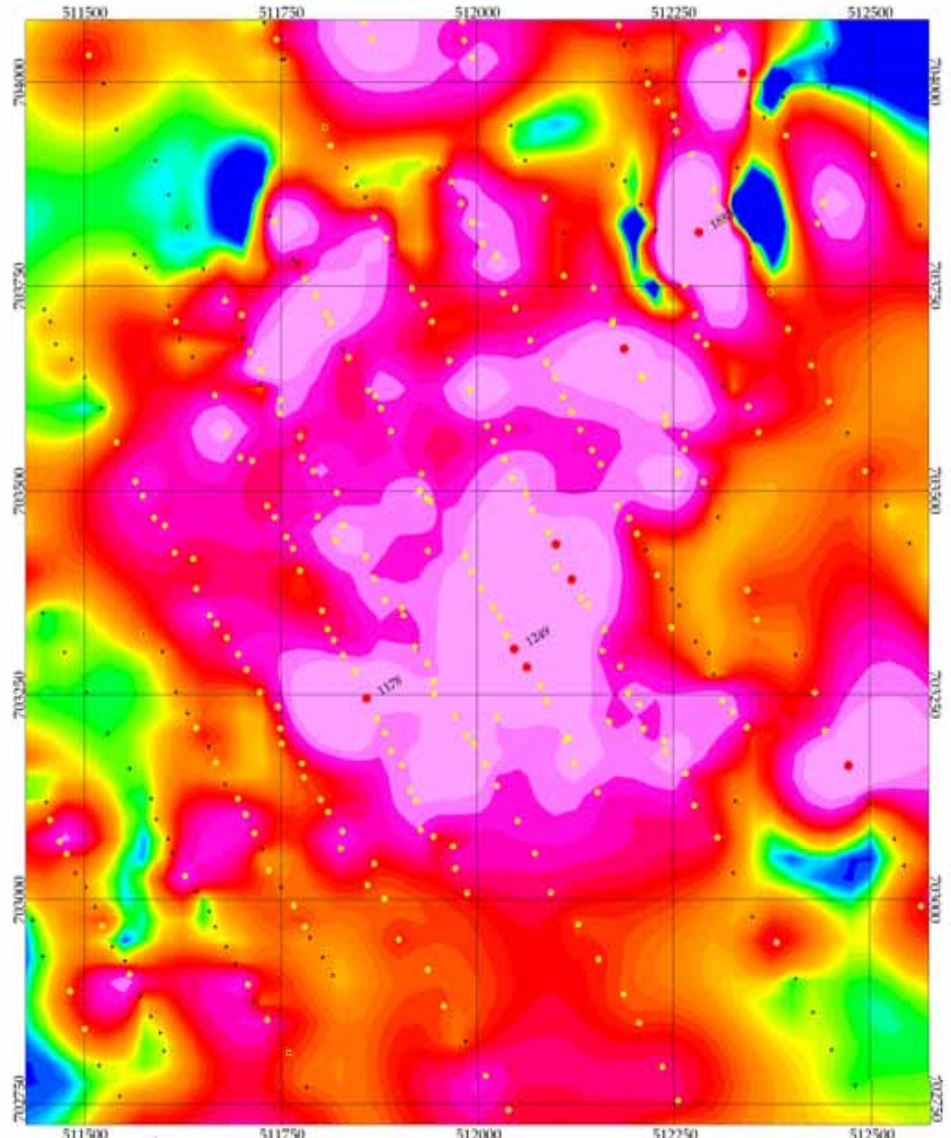
Boizan Prospect Gold Soil Geochemistry Sumiakrom Gold Anomaly
